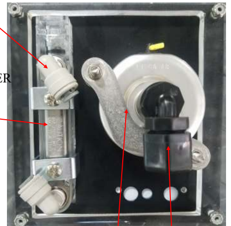
PRESSURE GAUGE PL-PSG-LP2.5
